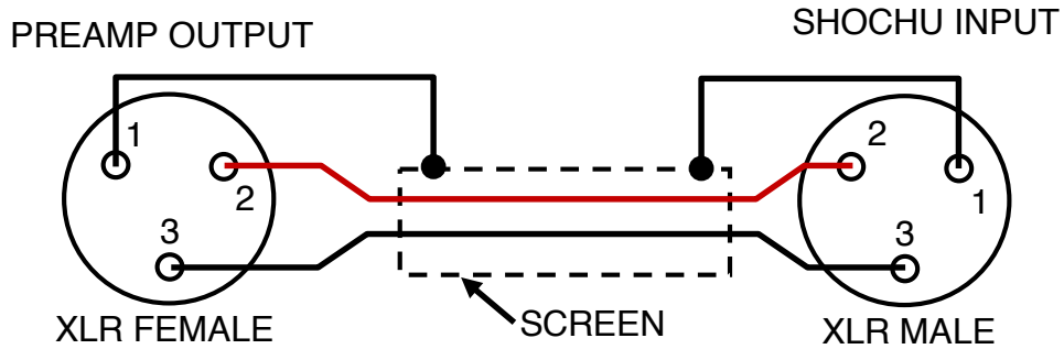
CONVENTIONAL: SCREEN CONNECTED AT BOTH ENDS
