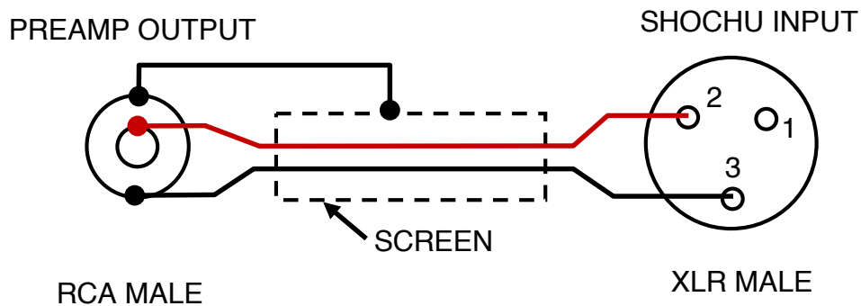
CABLE CONFIGURATION FOR RCA SINGLE ENDED PREAMP OUTPUT TO XLR BALANCED AMPLIFIER INPUT
